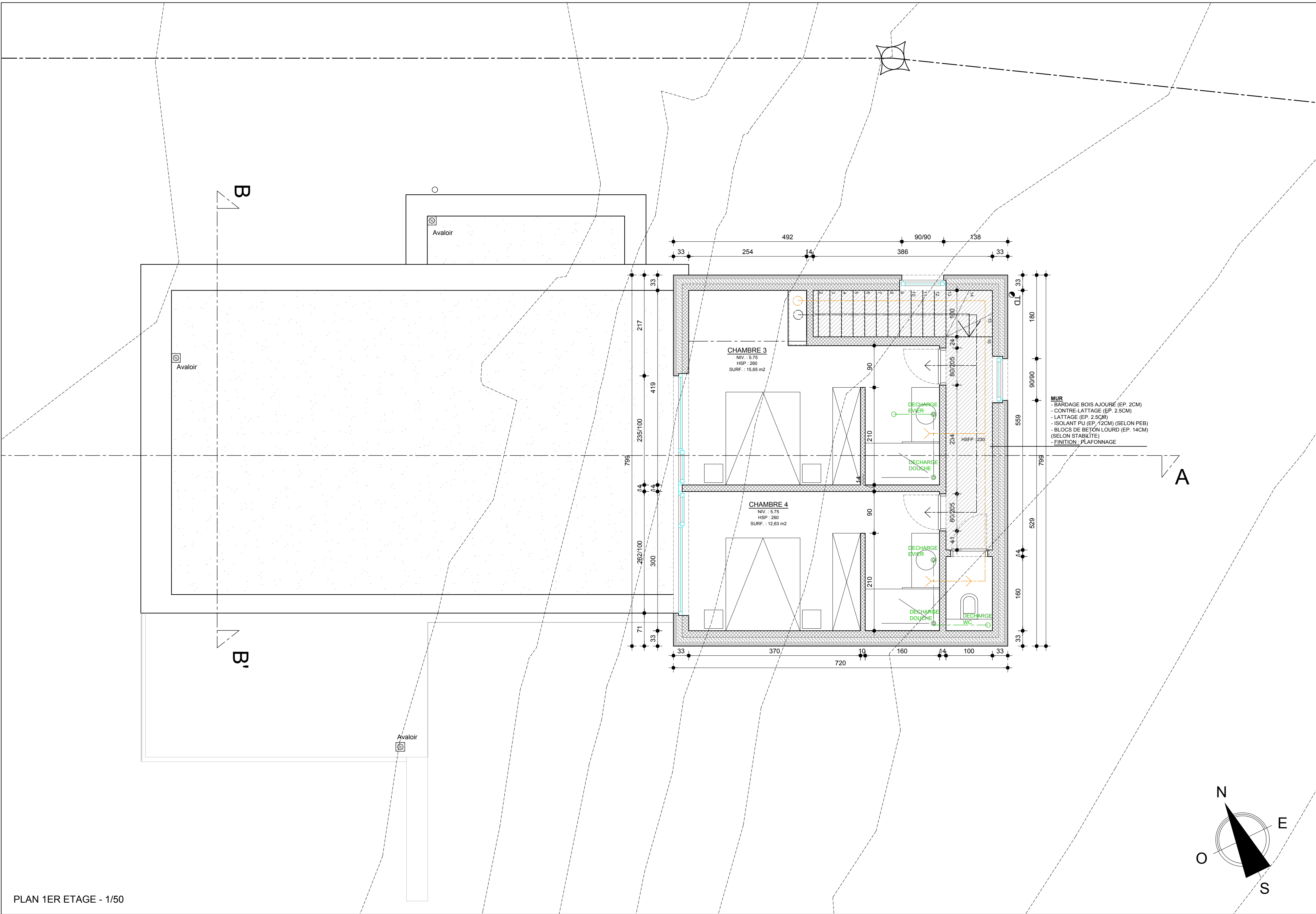
PLAN REZ-DE-JARDIN - 1/50
